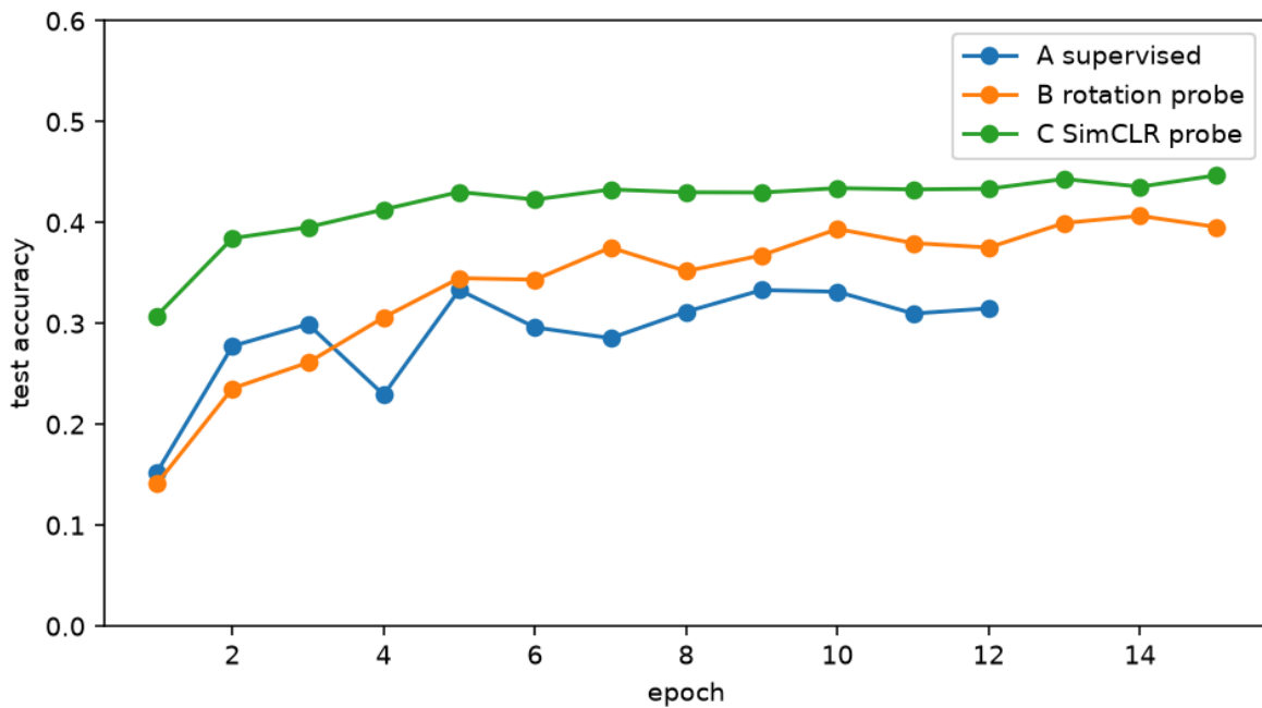
Test accuracy
