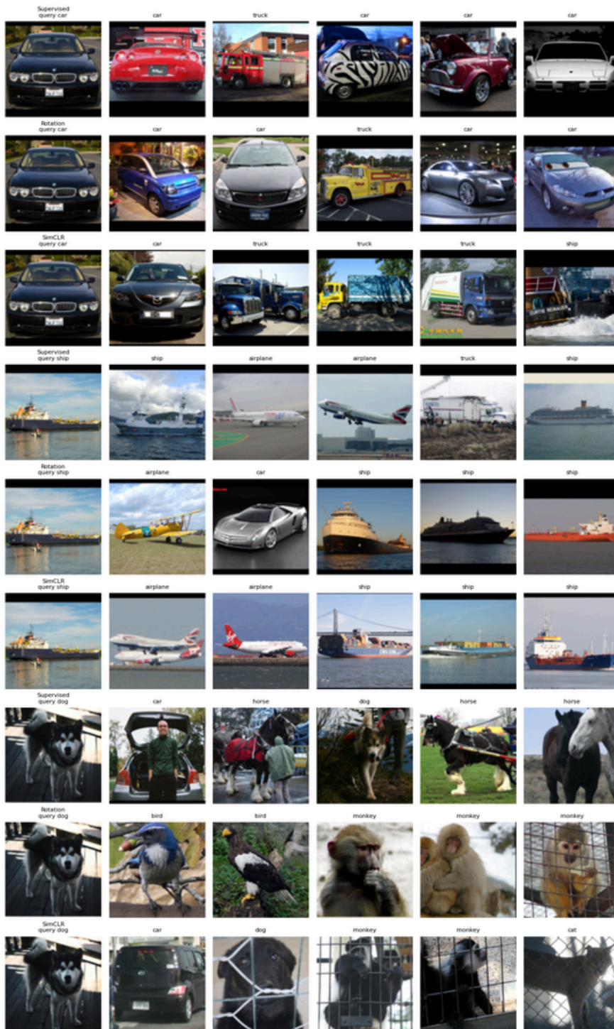
Nearest neighbors
