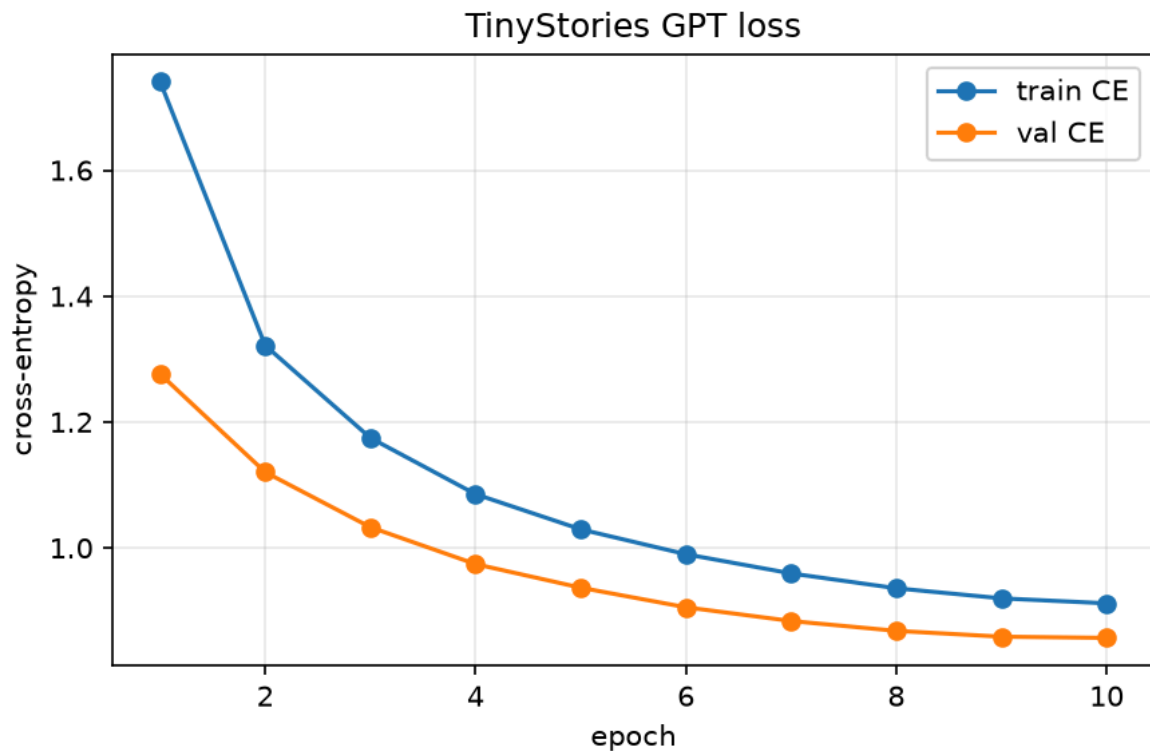
Part 1 training and validation loss
