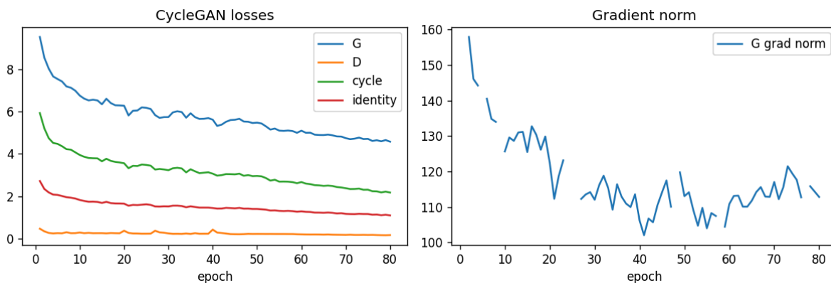
CycleGAN losses and gradient norm
