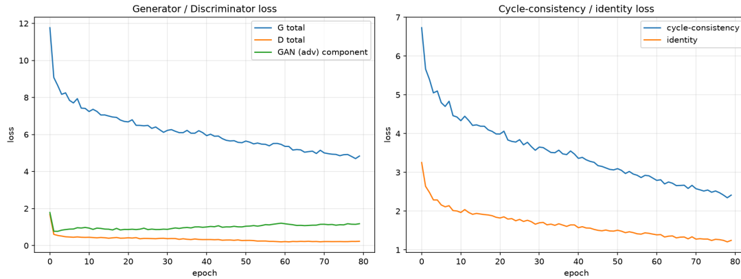
CycleGAN losses
