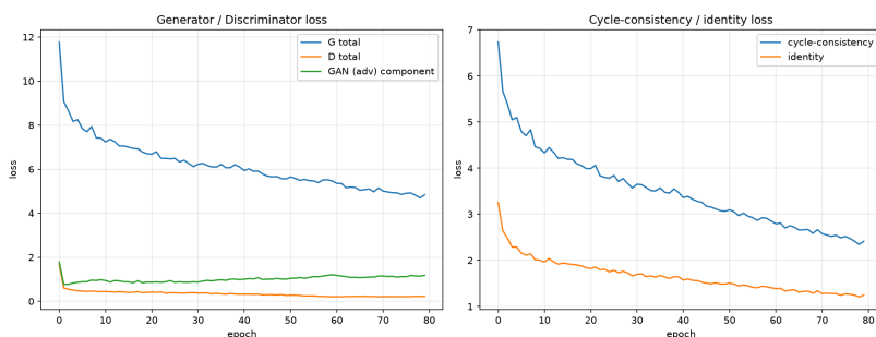
CycleGAN losses
