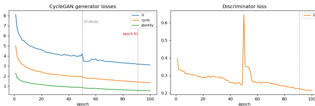
CycleGAN losses
