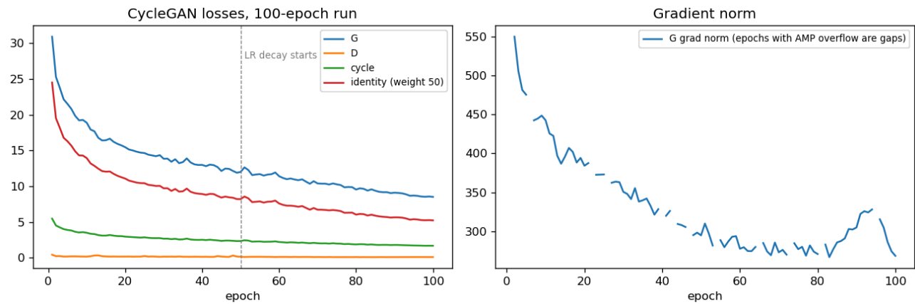
CycleGAN losses and gradient norm
