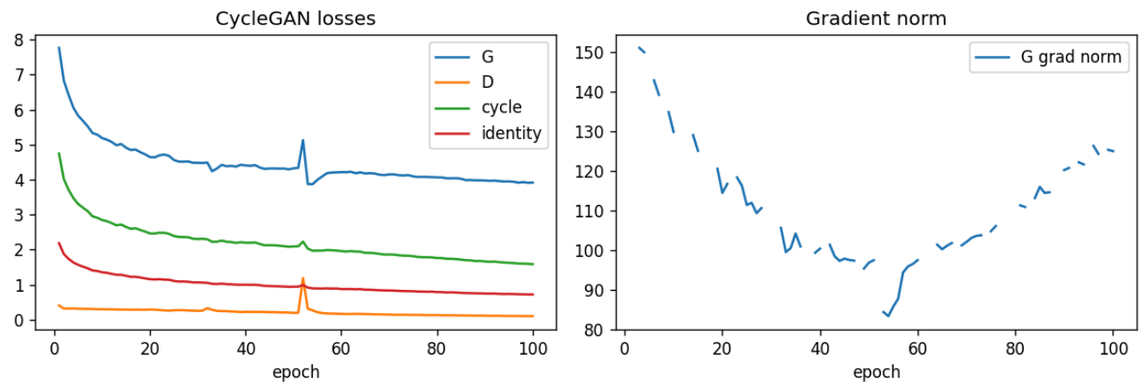
CycleGAN losses and gradient norm
