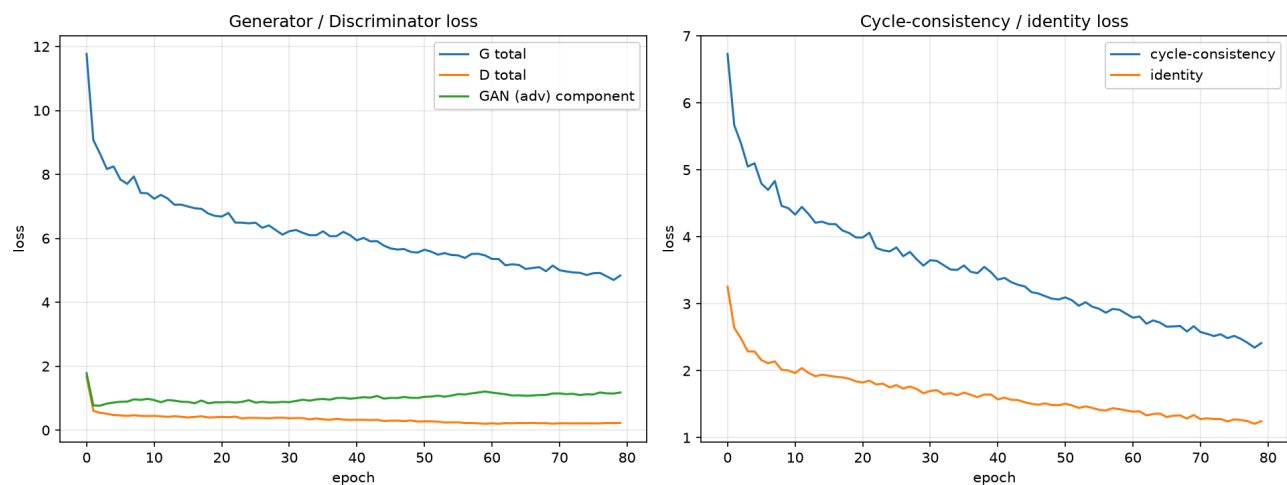
CycleGAN losses
