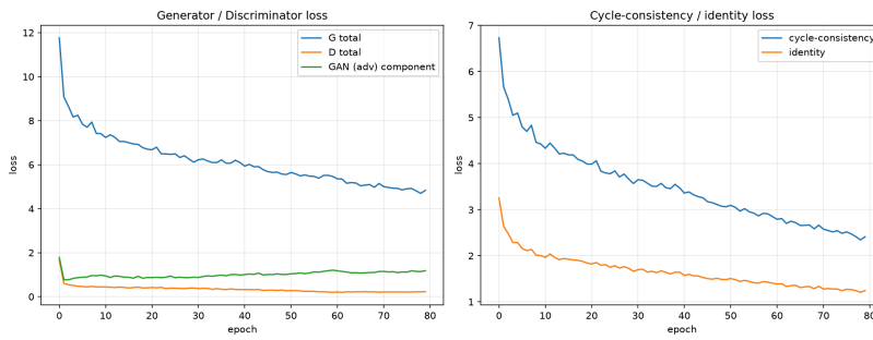
CycleGAN losses
