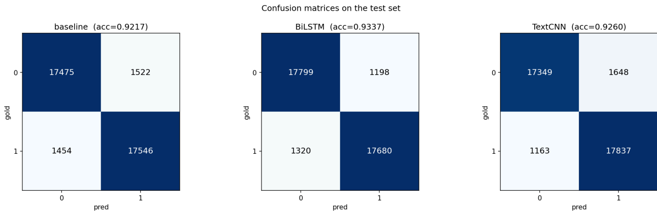
Baseline, BiLSTM and TextCNN confusion matrices (Ritika)
