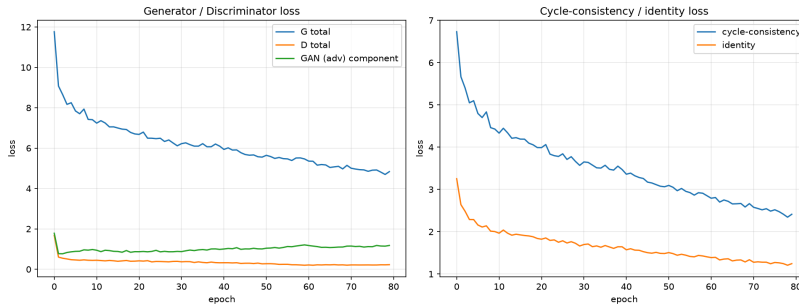
CycleGAN losses
