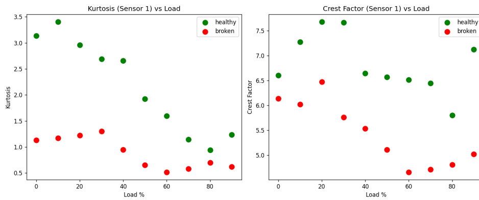
Figure 10: Kurtosis and crest factor separating Healthy vs. Broken Tooth across load levels
