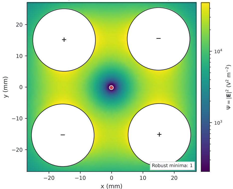
(b) Quadrupole connection: effective potential
