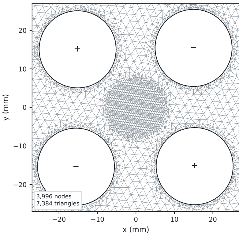
(a) Quadrupole connection: FEM mesh
