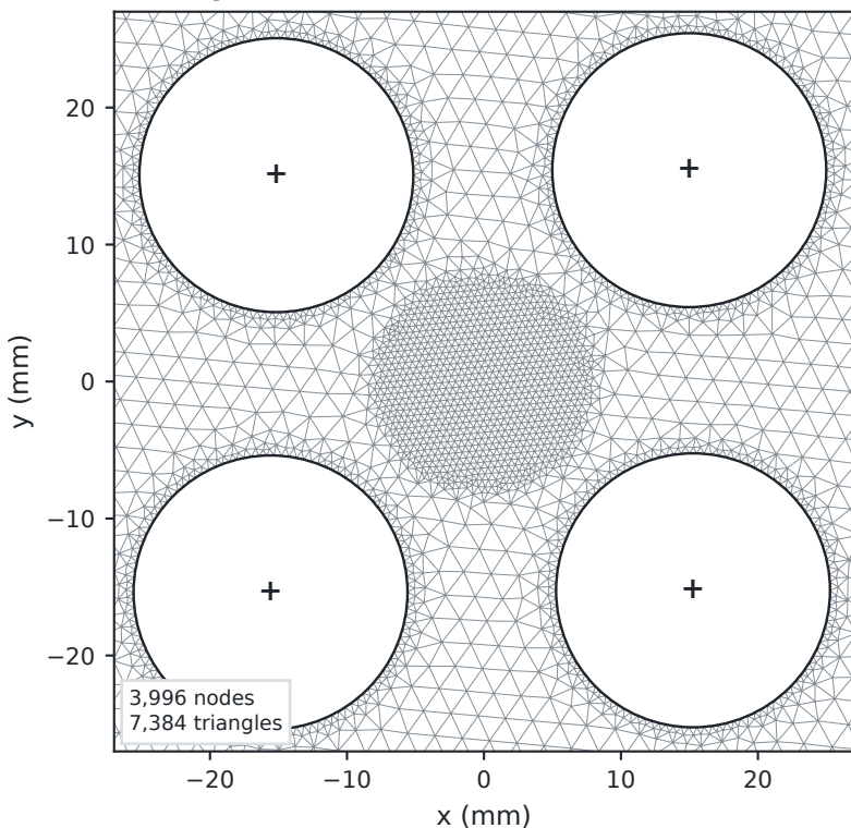
(c) In-phase connection: FEM mesh
