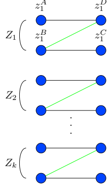
Figure 9.1: Worst case scenario for a deterministic cache algorithm
