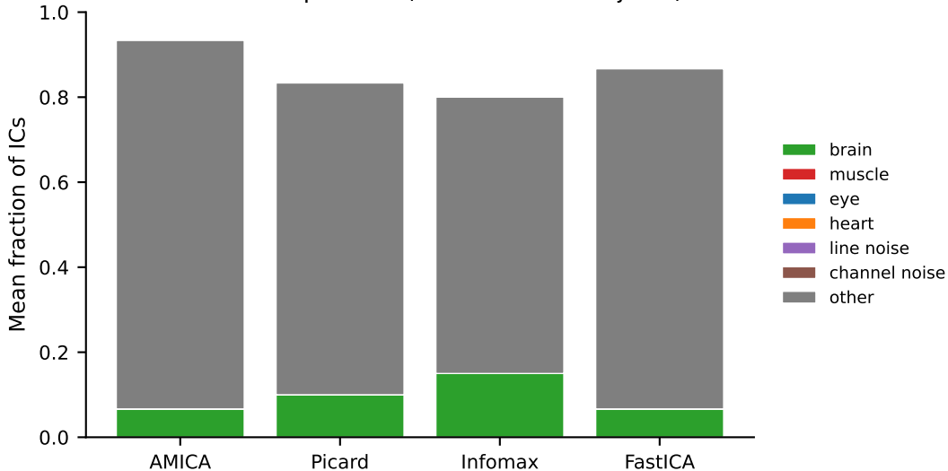
ICLabel composition (mean across subjects)
