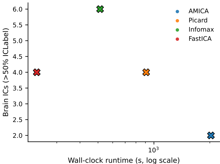
Runtime vs quality (paired by subject)
