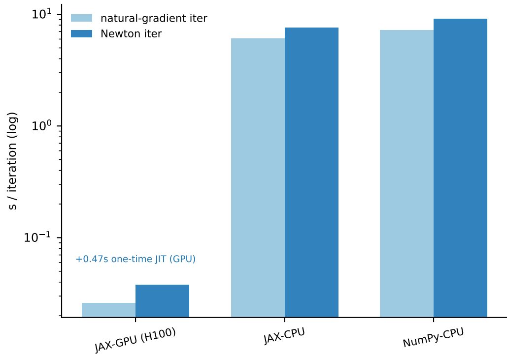
(B) Natural-gradient vs Newton per-iteration cost
