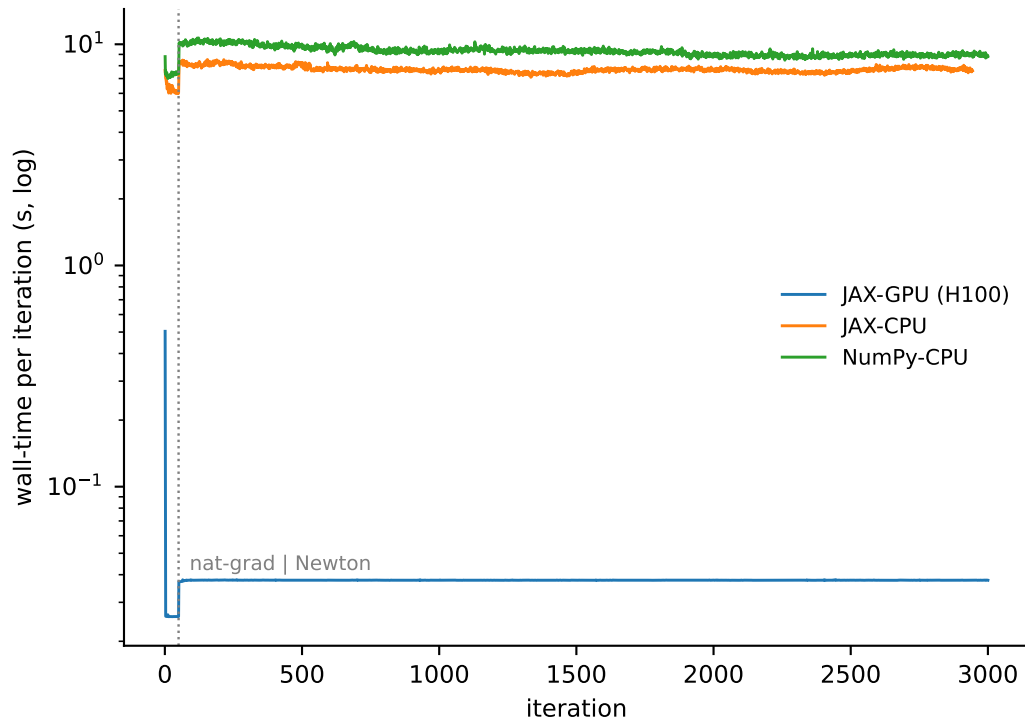
(A) Per-iteration cost (mean over subjects)
