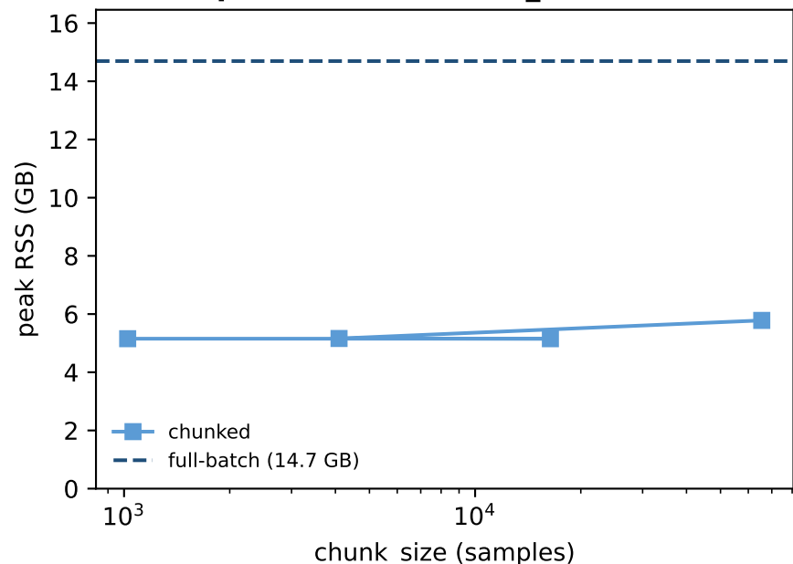
B. CPU peak RSS vs chunk_size (T=785k) — bounded
