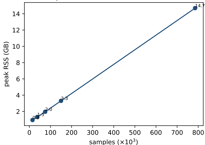
A. CPU peak RSS vs T (full-batch) — \sim O(T)
