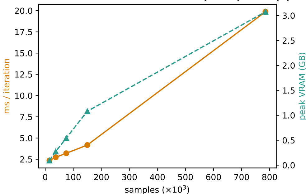
C. GPU runtime + VRAM vs T (C=64) — \sim O(T)
