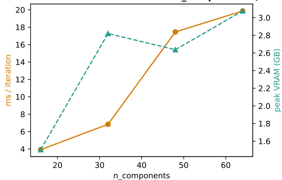
D. GPU runtime + VRAM vs n_components (T=785k)
