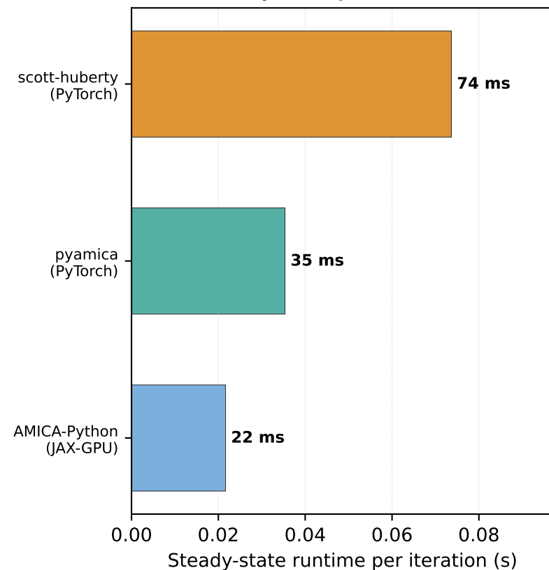
C. GPU steady-state per iteration (H100)
