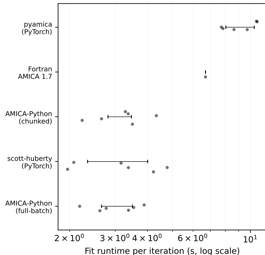
B. CPU runtime distribution
