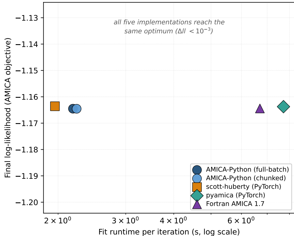
A. Quality-cost (ds004505 sub-01): same optimum, different speed
