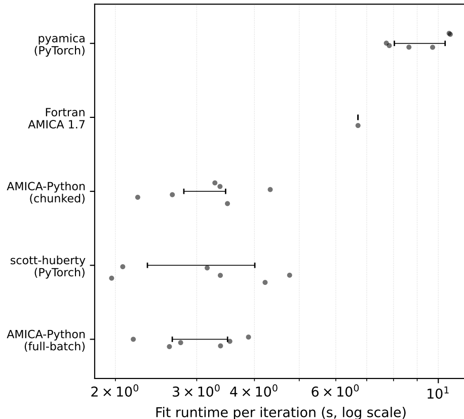
B. Per-implementation runtime distribution
