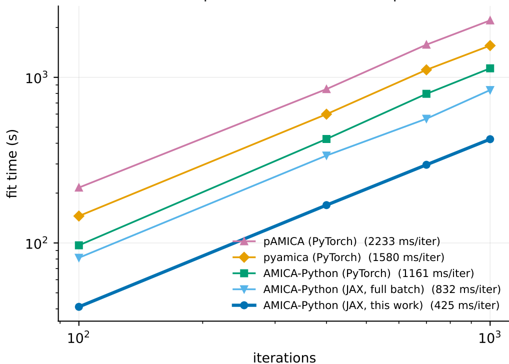
Local CPU — i7-10750H, 6 cores 30 components x 166,800 samples
