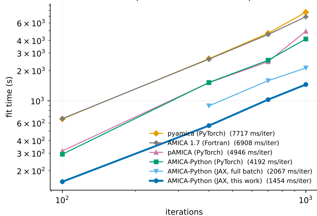
Cluster CPU — EPYC 9655, 8 cores 64 components x 785,328 samples
