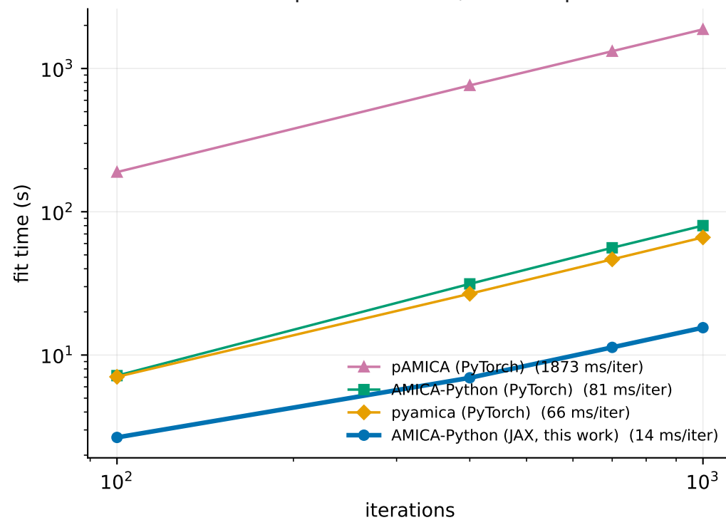
Cluster GPU — one H100 64 components x 785,328 samples
