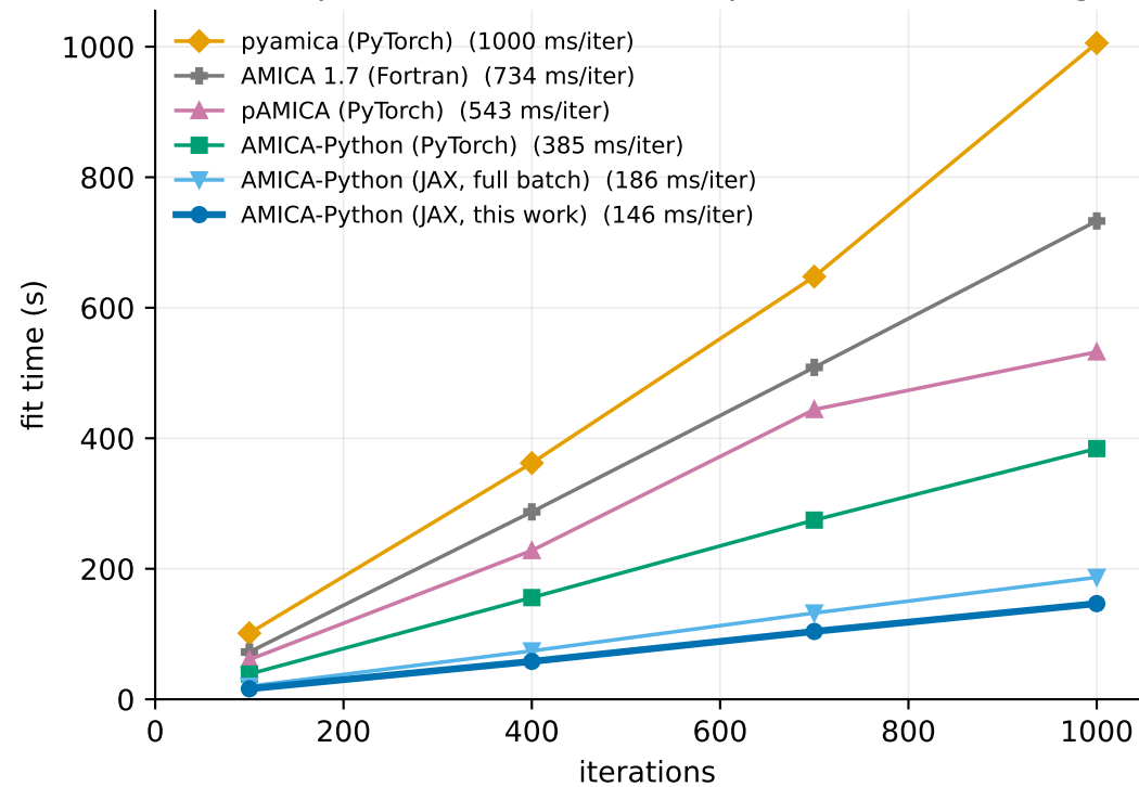
Cluster CPU — EPYC 9655, 8 cores 30 components x 166,800 samples (same recording)
