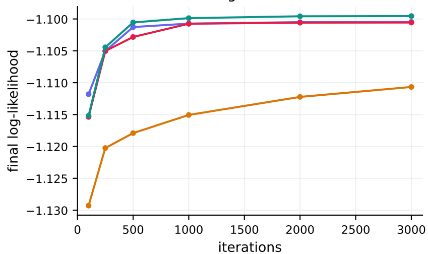
CPU · convergence vs iterations
