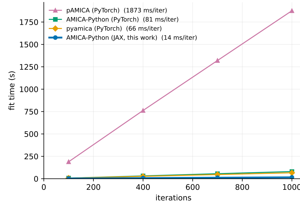
Cluster GPU — one H100 64 components x 785,328 samples
