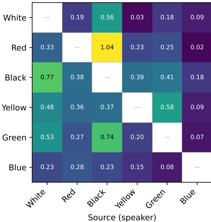
BEAR-guided diffusion
