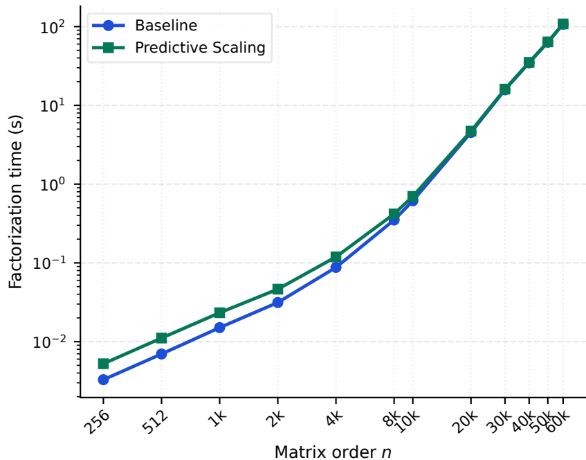
(a) Factorization Time
