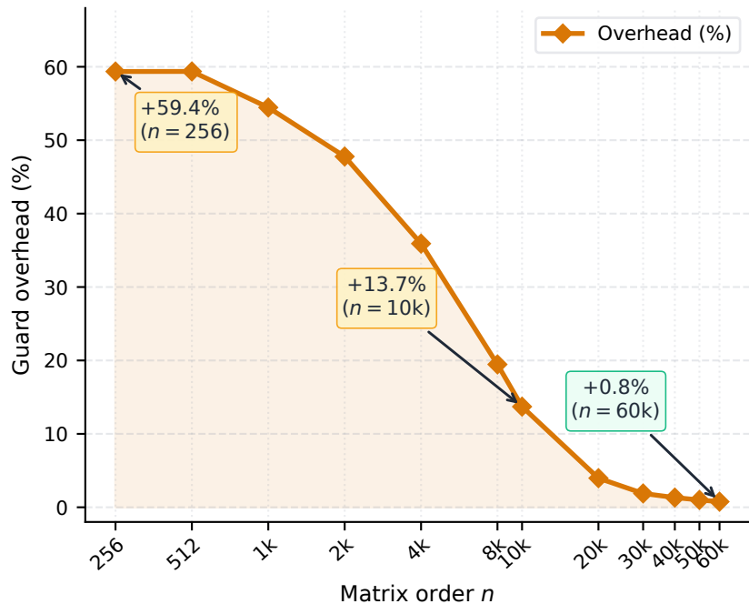
(b) Predictive Guard Overhead
