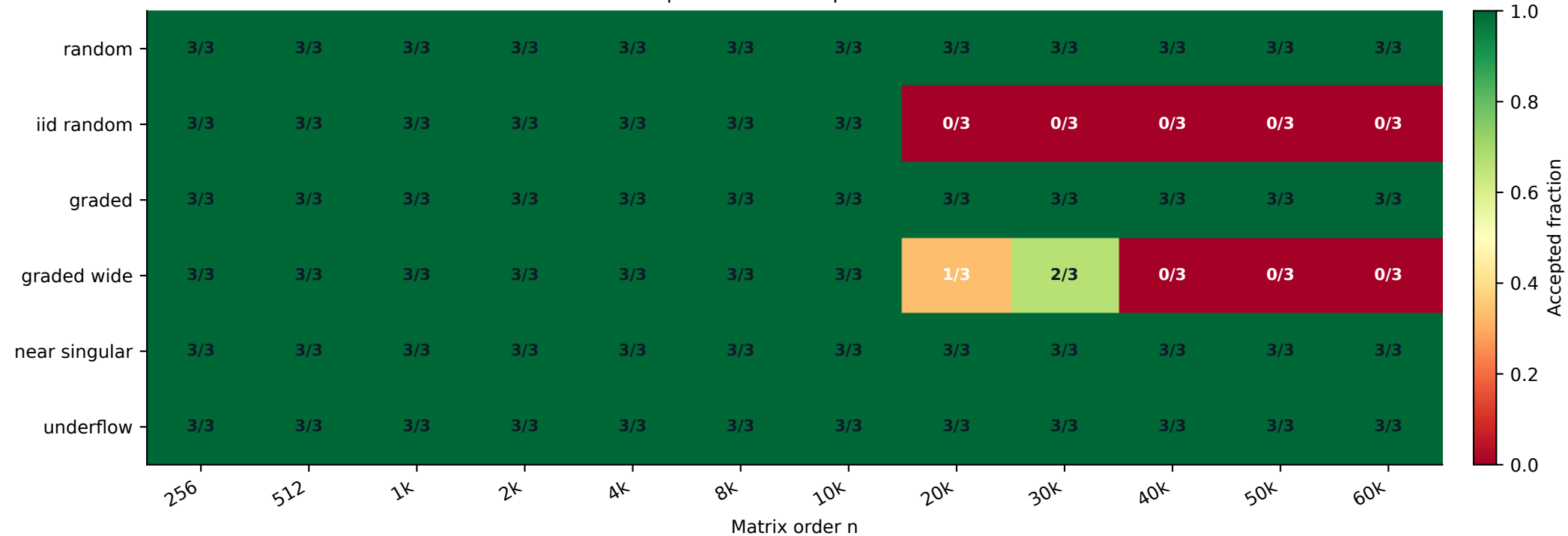
Predictive completion with sampled residual below one
