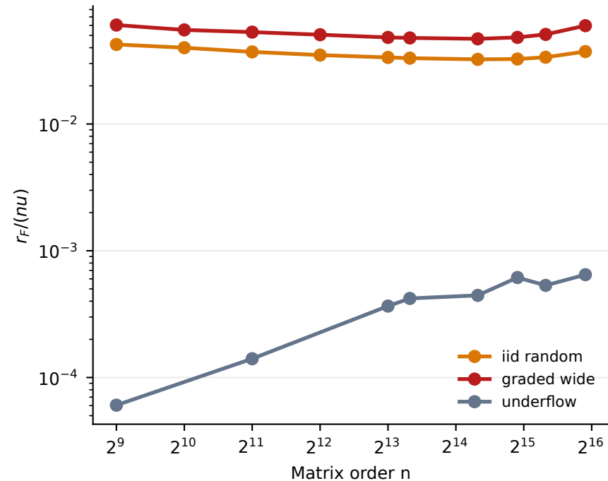
Normalized FP16 precision wall
