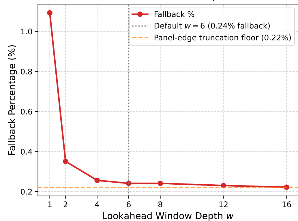
(c) Fallback Rate vs. Lookahead Depth w ( \tau = 1.01 )
