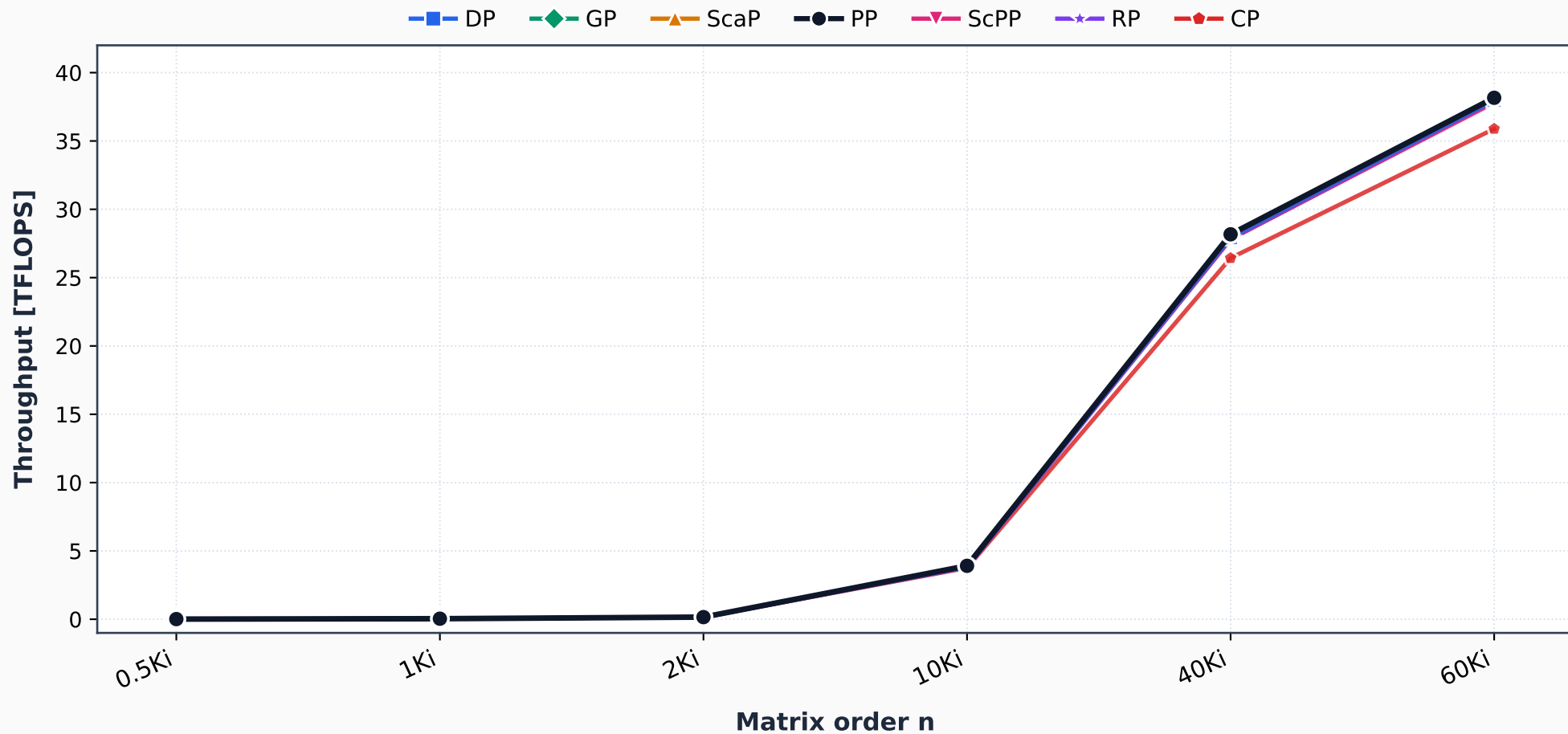
Throughput across matrix dimensions
