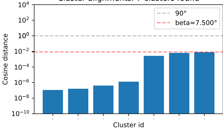
Cluster alignments: 7 clusters found
