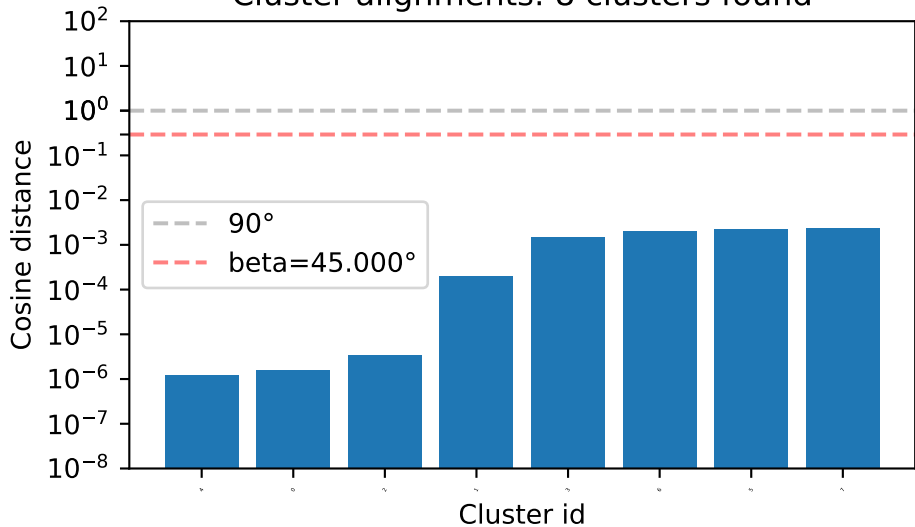
Cluster alignments: 8 clusters found
