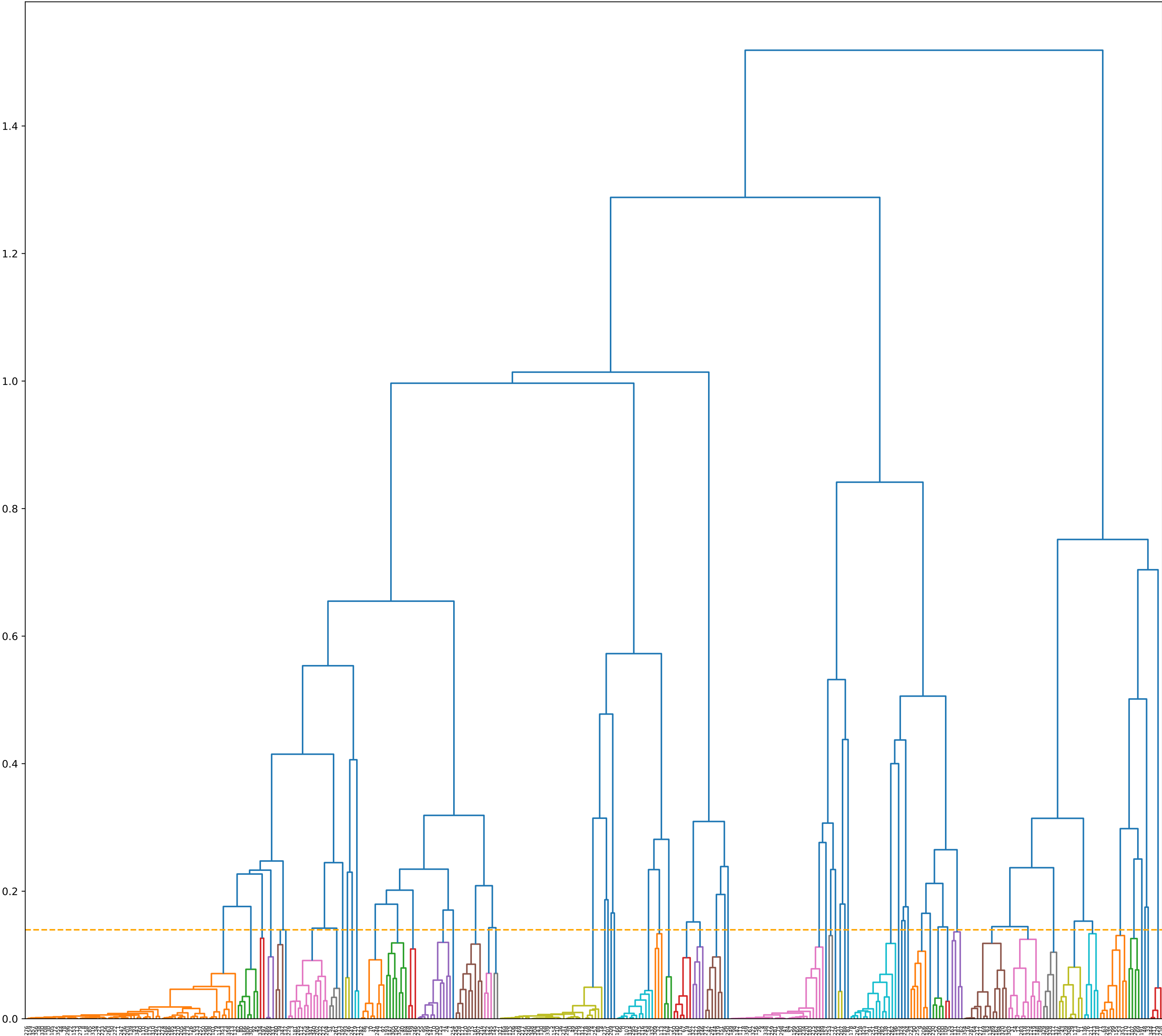
average linkage
