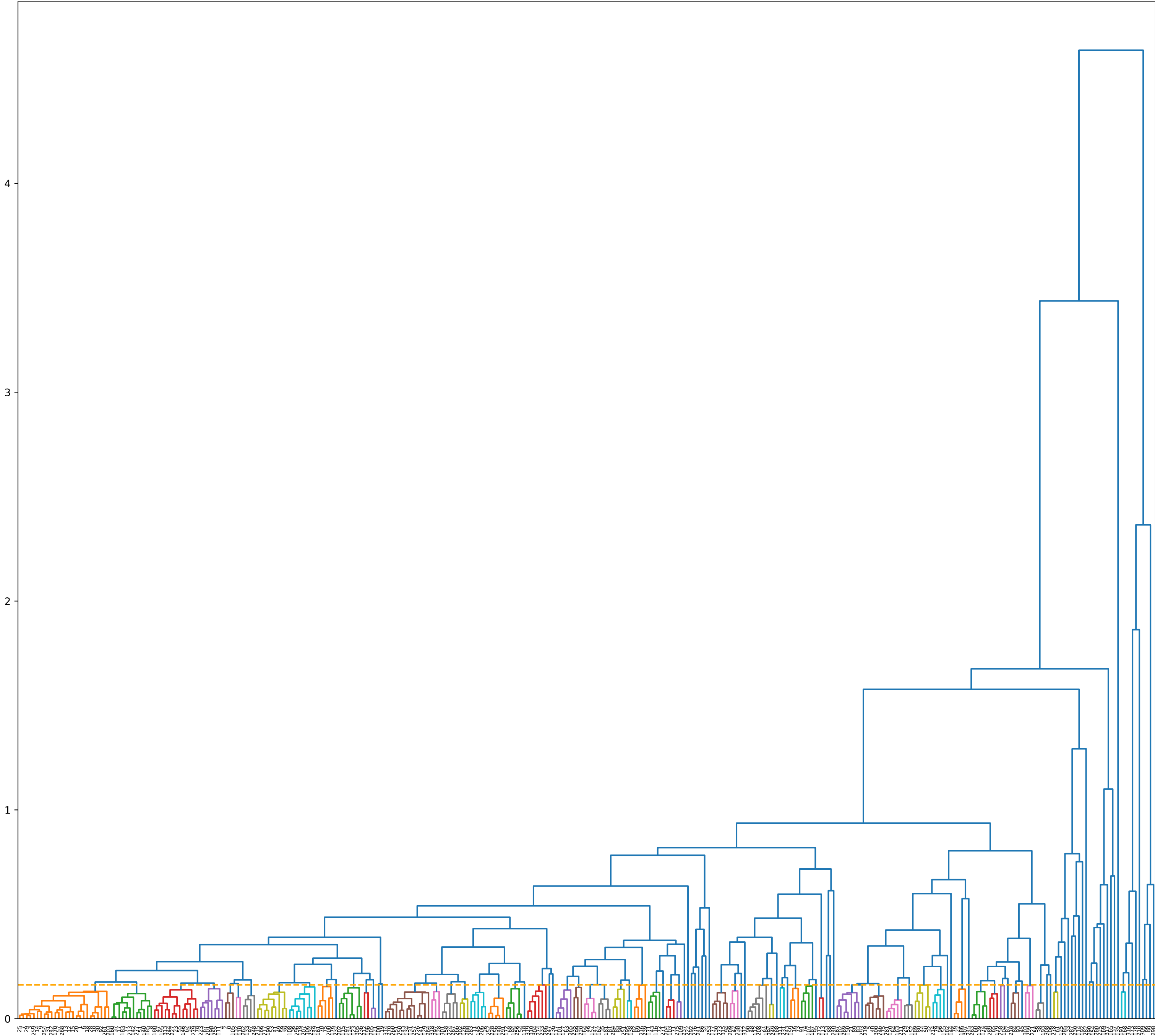
average linkage
