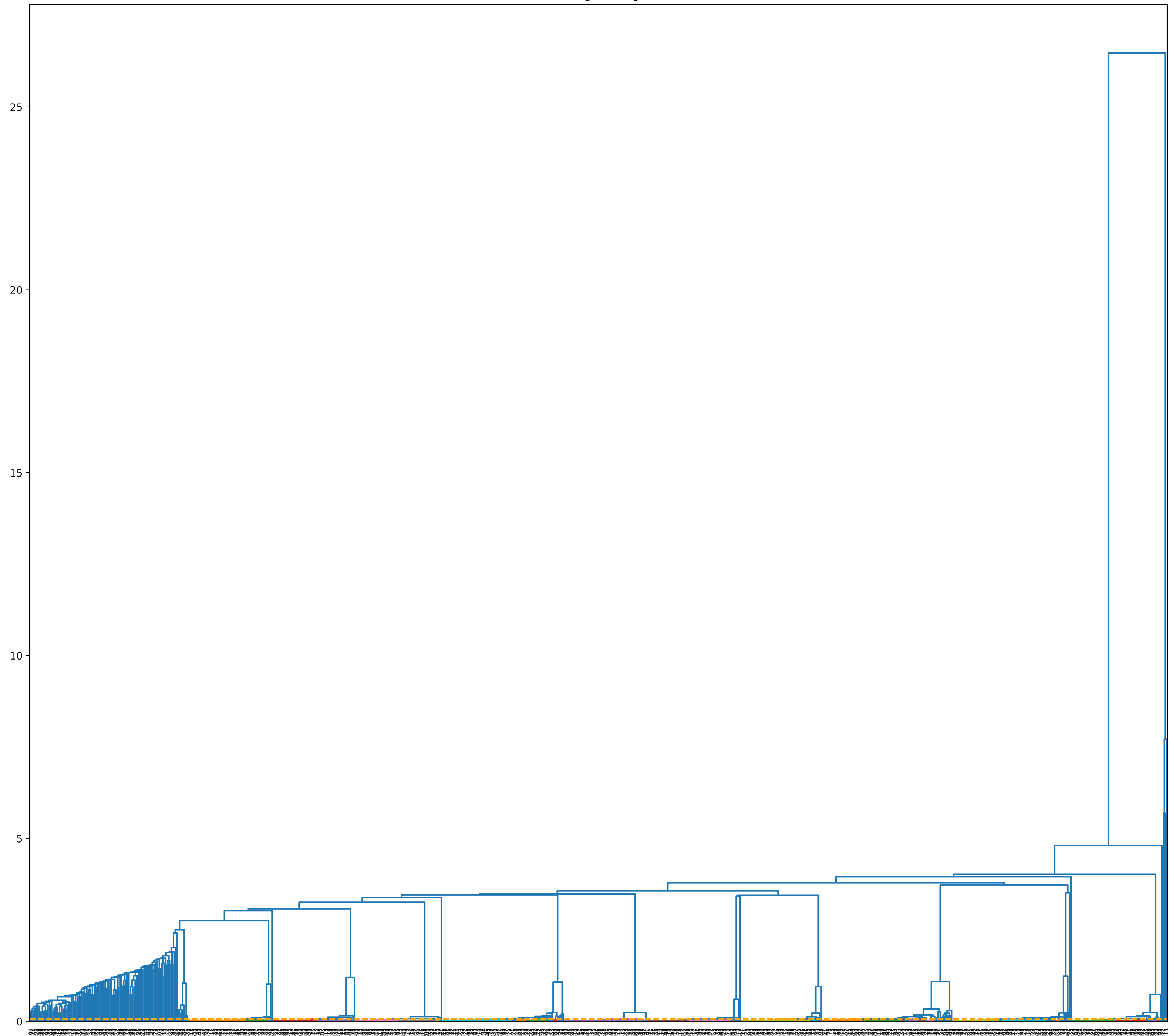
average linkage
