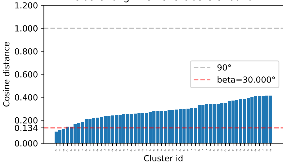
Cluster alignments: 3 clusters found
