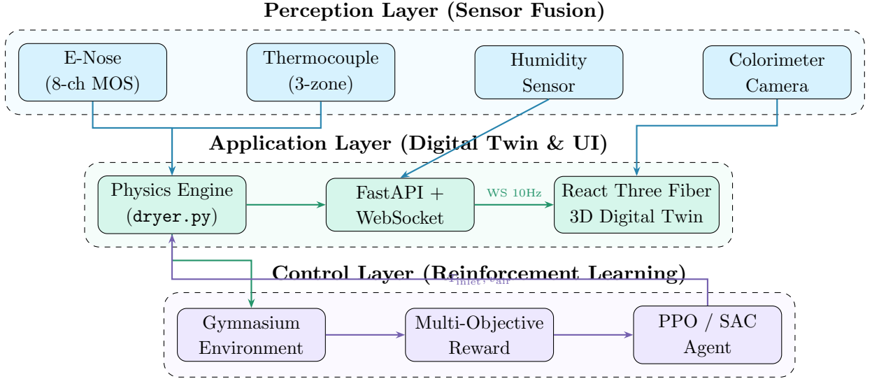
Figure 4.1: NeuraLeaf three-layer system architecture showing data flow from sensors through the Digital Twin to the RL controller and back.
