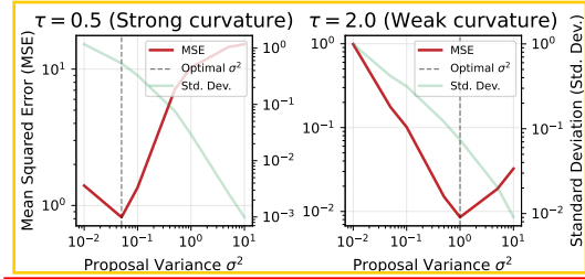
Figure 2: Mean-squared error and standard deviation of the FSM estimator \tilde{S} with varying proposal hyperparameter \sigma^2 , for two Gaussian likelihoods \mathbf{x} \sim \mathcal{N}(\theta, \tau^2) with differing curvature.
