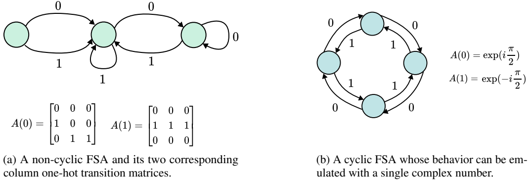
Figure 2: Any N -state FSA can be encoded using sparse binary N \times N transition matrices (a), but modular counters admit a more compact representation based on diagonal transition matrices (b).
