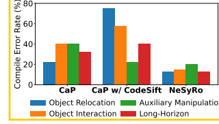
Figure 4: Real-world compile error rate over all task types
