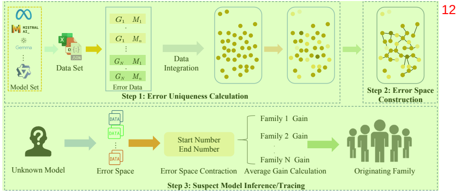
Figure 3: The overview of error space-based traceability mechanism ErrorTrace.
