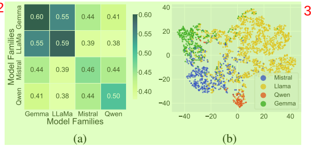
Figure 1: (a) Intersection of erroneous data from different family models. (b) Error space dimensionality reduction display.
