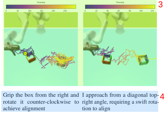
Figure 5: Conditional behavior generation. Figures in the right panel show generated behaviors for the specified condition as inner speech with no subsequent updates.
