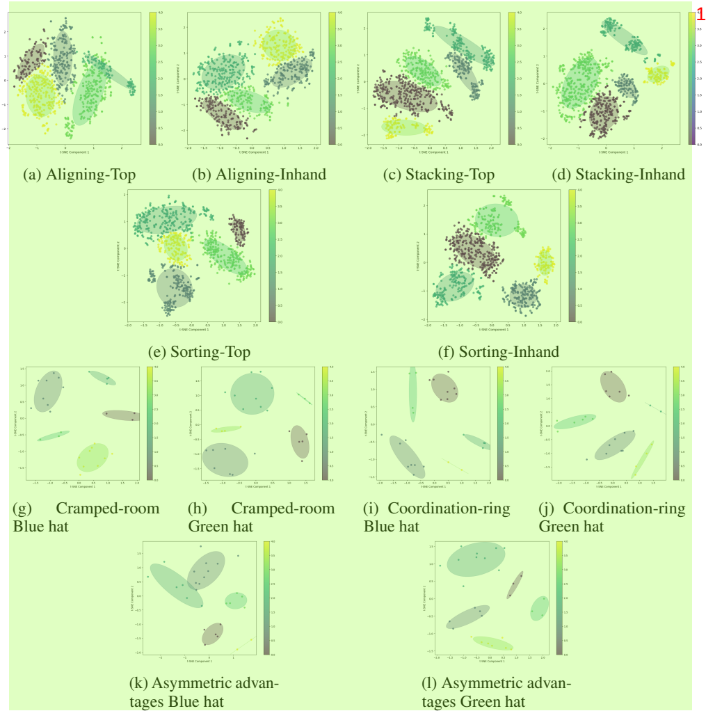
Figure 8: TSNE visualization of CLIP-encoded inner speech generated using GPT-4o for the environments used in our experiments. (a-f): Top and inhand cameras in D3IL: Aligning, Stacking and Sorting environments, respectively. (g-l): Blue and green hat agents in overcooked map layouts: Cramped-room, Coordination ring, and Asymmetric Advantages, respectively.
