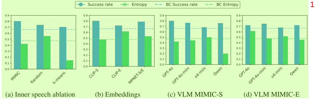
Figure 4: Effect on Success Rate and Entropy performance of MIMIC on changing various components on the Aligning dataset: (a) removing inner speech during simulation, (b) changing the embedding model, (c-d) using different VLMs for training and scaffolding.
