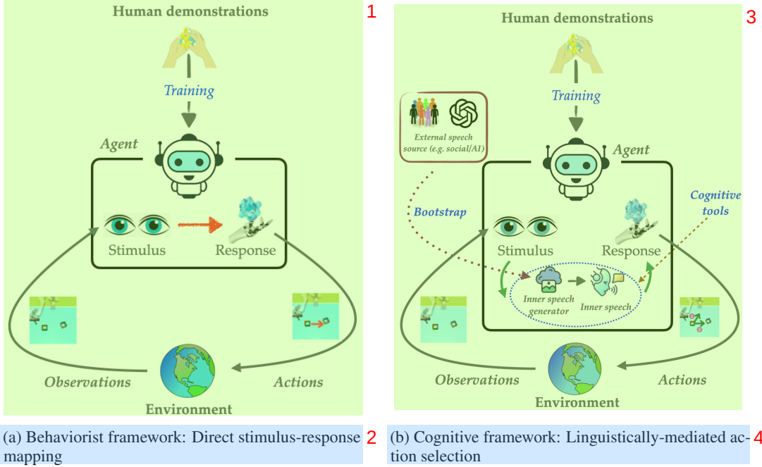
Figure 6: Contrasting theoretical frameworks for IL. (a) The behaviorist approach models human behavior as a direct mapping from environmental states to actions ( s_t \mapsto_{\mathcal{H}} a_t ), treating cognitive processes as opaque transformations. (b) The cognitive approach instantiated by MIMIC introduces inner speech as a mediational layer ( s_t \rightarrow m_t \rightarrow a_t ), where m_t represents linguistically-structured internal deliberation that enables behavioral diversity and contextual adaptation.
