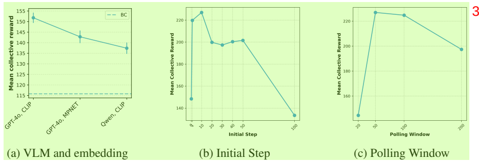
Figure 10: Sensitivity on overcooked Cramped-room 4
