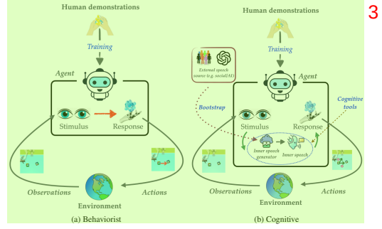
4 Figure 1: Paradigm comparison. (a) direct state-to-action mapping. (b) inner speech m_t mediates between perception and action. Extended discussion available in Appendix B.1.
