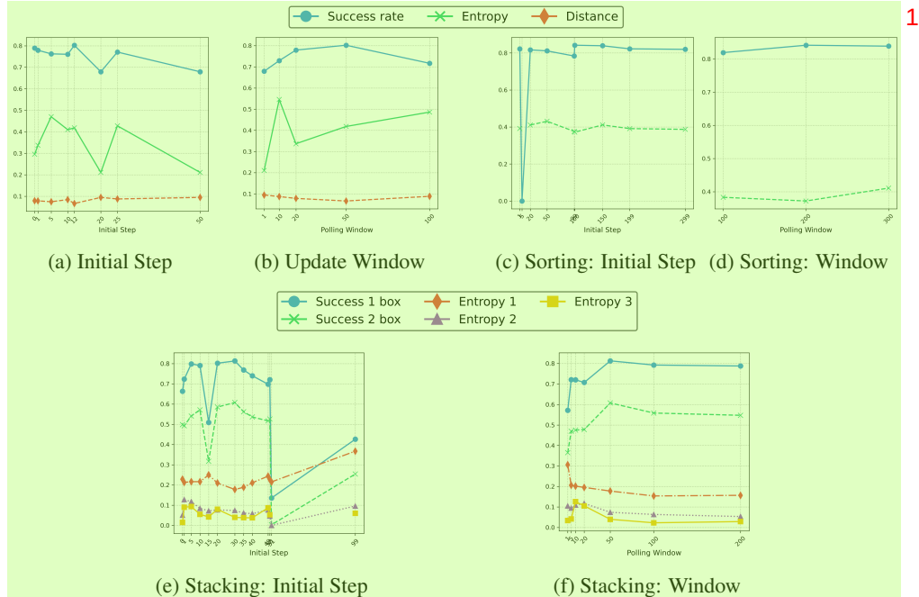
Figure 9: Hyperparameter sensitivity of MIMIC on the D3IL benchmark. 2
