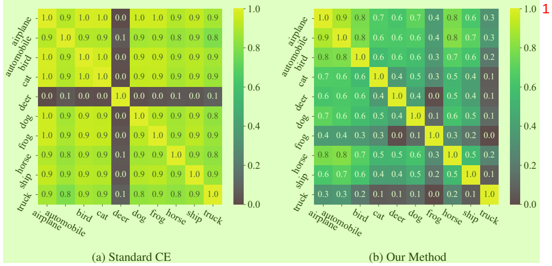
Figure 4: Class-level feature representation cosine similarities on CIFAR-10-LT (IR=1000). (a) Standard cross-entropy loss. (b) Our proposed method, showing improved class separability.
