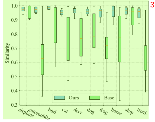
(b) Cosine similarity between original and augmented sample features on CIFAR-10-LT (IR=10, trained on IR=1000). Our method shows higher robustness.
