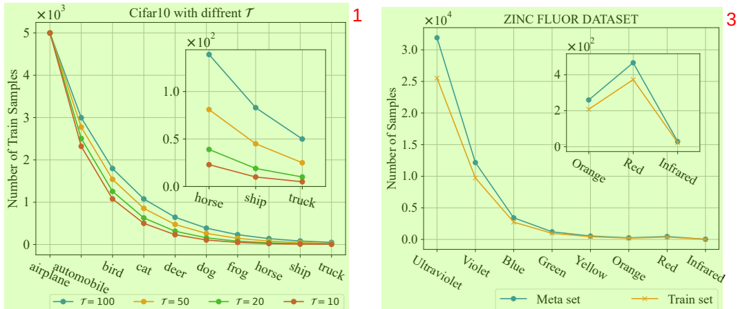
(a) Training sample distribution per class in CIFAR-10-LT under different \mathcal{T} settings. (b) Comparison of meta-samples per class with training samples in ZincFluor .
