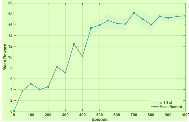
Figure 6: The convergence of RL in the HM3 at the architecture space. 4
