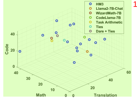
Figure 4: The illustration of different model merging methods in the text translation, math reasoning, and code generation tasks.
