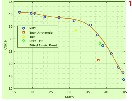
Figure 5: The illustration of different model merging methods in the math reasoning and code generation tasks.
