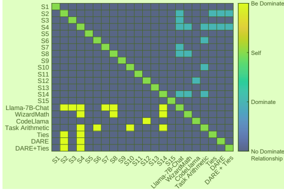
Figure 2: Illustration of metrics for different merging methods, where S1 represents solution1 obtained by HM3. 4
