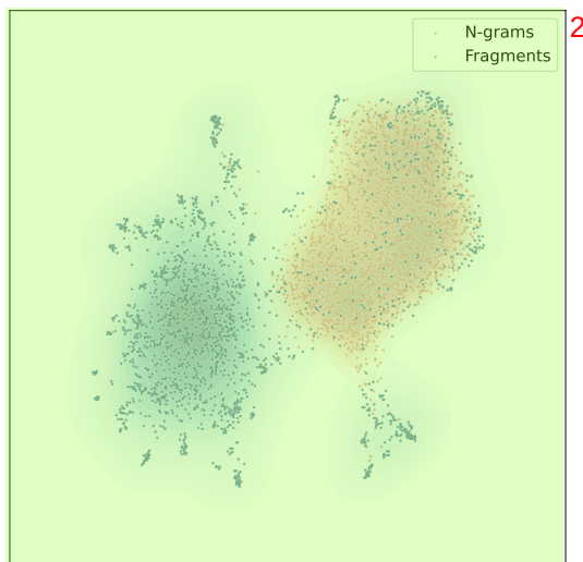
Figure 15: Visualization of fragment and N-gram embeddings represented by the Fragment Encoder.
