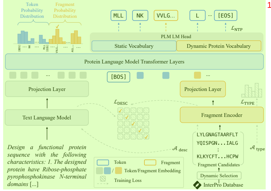
Figure 3: Overview of our model architecture.
