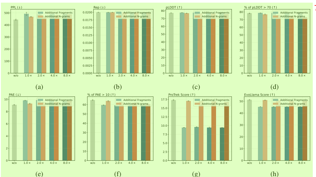
Figure 14: Results of incorporating additional fragments or N-gram subsequences during inference. The experiments are conducted under the setting of K = 32 . Gray bars indicate the performance of retrieving the top 32 relevant descriptions without incorporating any additional fragments or N-grams. The x-axis represents the multiple of noise introduced relative to the original number of fragments during inference.
