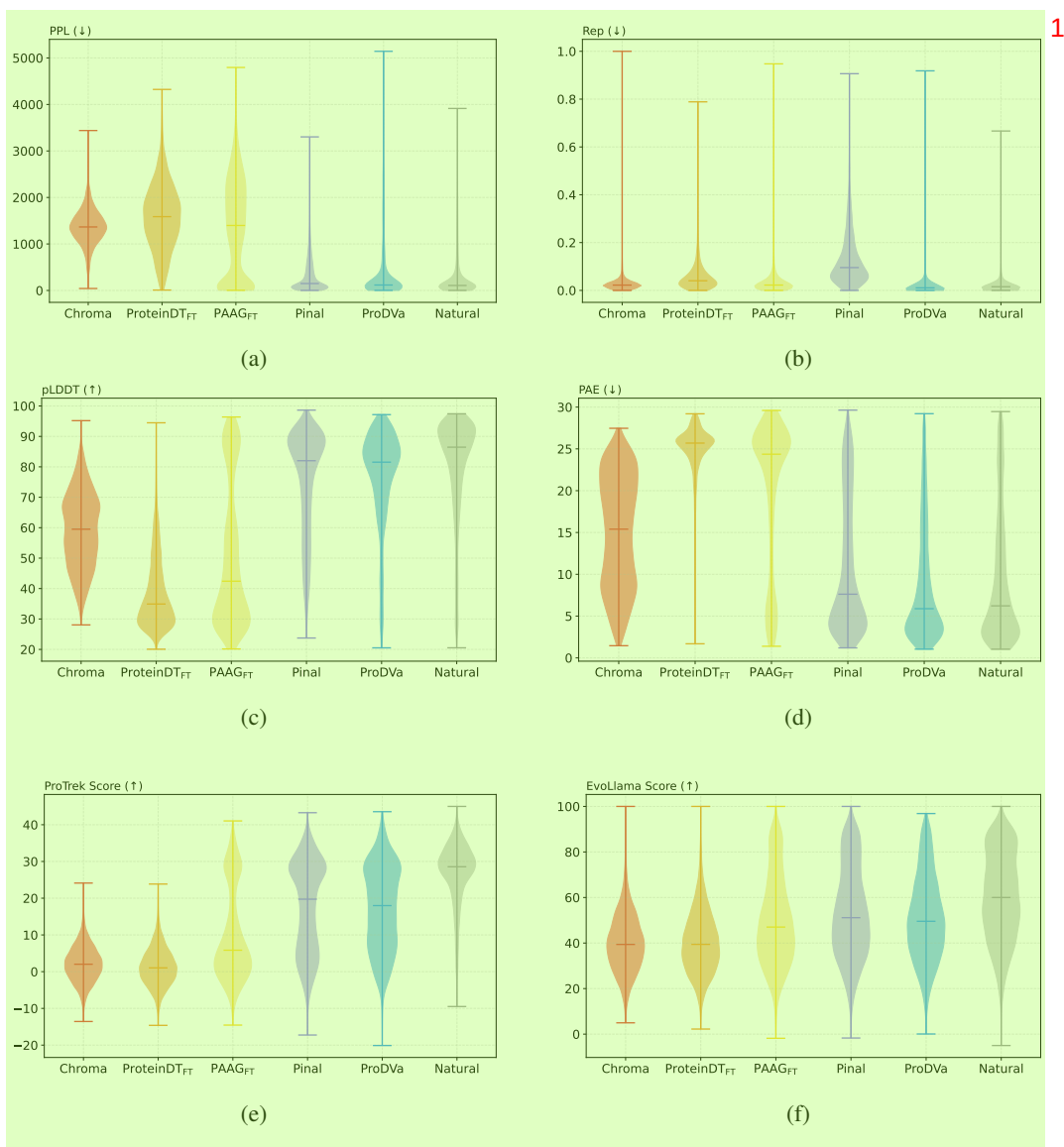
Figure 12: Violin plots illustrating the results on the Mol-Instructions protein design task. 2
