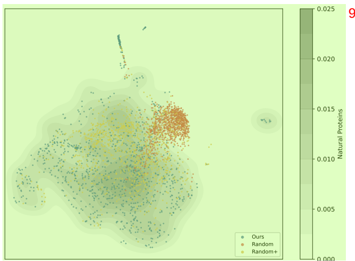
Figure 8: Additional visualization of proteins designed by our method, Random, and Random+, embedded using Pinal (SaProt module) and projected with UMAP. 10
