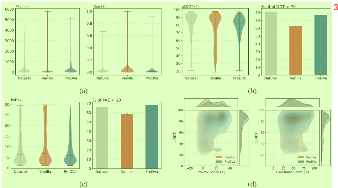
Figure 4: Experimental results comparing PRODVA with a vanilla multimodal baseline on Mol-Instructions. (a) illustrates performance on sequence plausibility metrics. (b) and (c) show performance on foldability metrics. (d) presents performance on language alignment metrics, where deeper colors in the upper right corner indicate better performance. 4
