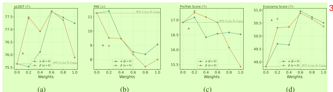
Figure 9: Evaluations on the effect of loss weighting. The blue lines indicate the effect of \alpha with \beta = 0 , while the red lines indicate the effect of \beta with \alpha = 0 . The triangle and star markers indicate configurations where both \alpha and \beta are set to 0.1 and 0.2, respectively. The grey dashed line denotes the performance without incorporating type loss and description loss during training.
