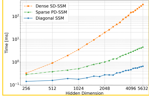
Figure 4: Runtimes of single-layer SSMs with varying dimension and sequence length 64.
