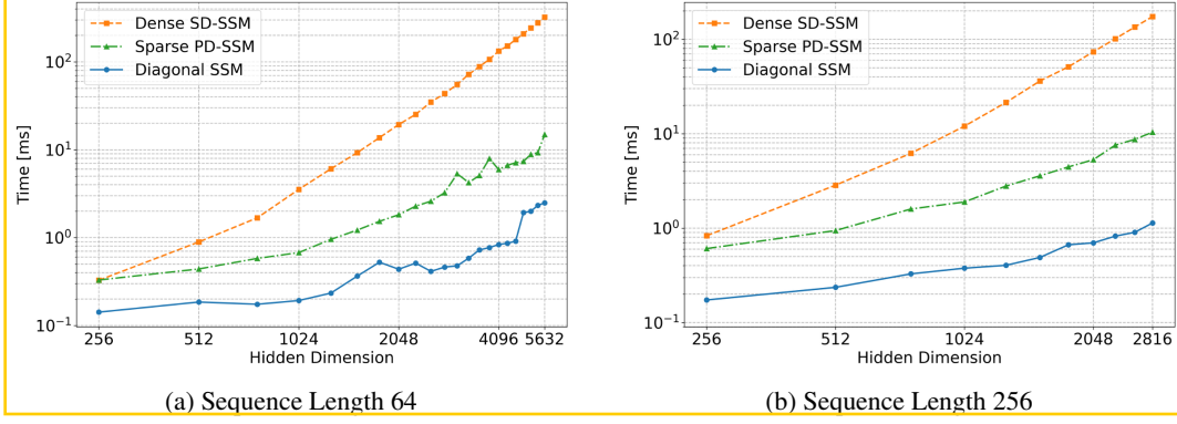
Figure S12: Runtime measurements in a parameter-matched setting.
