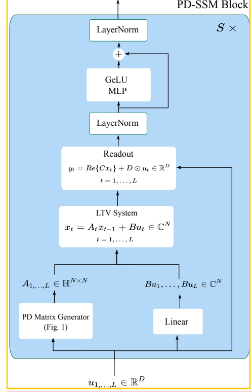
(b) Full PD-SSM model with a nonlinear readout, as used in the LRA and time-series experiments.
