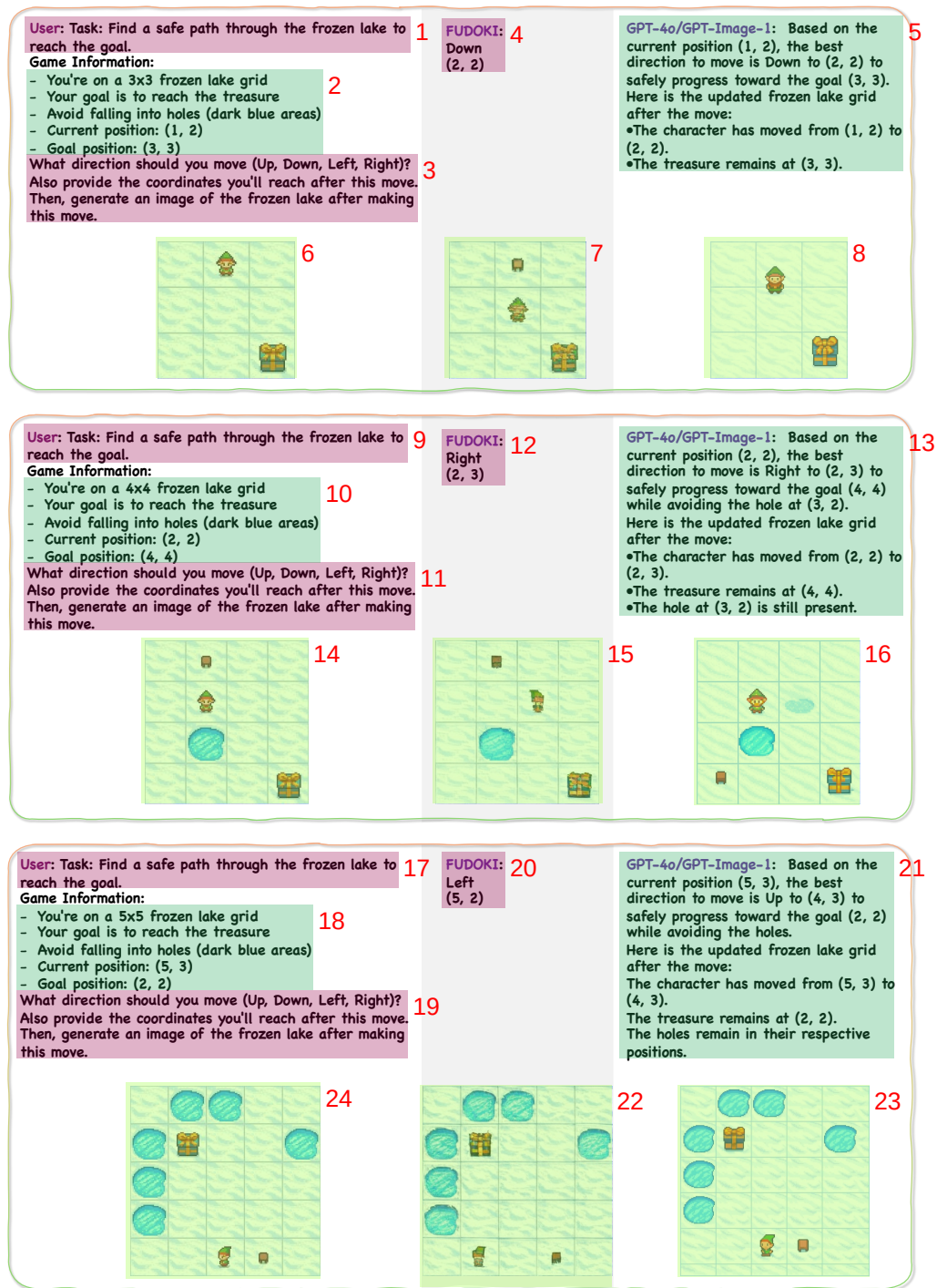
Figure 9: Comparison of FUDOKI and GPT-4o/GPT-Image-1 on frozen lake maze navigation tasks. GPT-4o/GPT-Image-1 offered well-reasoned textual outputs with safety and goal awareness but generated inconsistent visuals, even altering the maze (e.g., the third row). FUDOKI, by contrast, consistently produced valid directions and coherent visual updates aligned with task constraints, demonstrating stronger spatial consistency.
