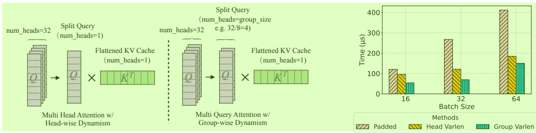
Figure 13: Left: Head-wise/group-wise varlen attention with flattened paged KV cache in Twilight. 12 Right: Comparison among the three attention methods on a real budget distribution of a LLaMA-3.1-7B layer on a 16k retrieval task. Here “Padded” means padding all heads to the maximum budget length; “Head Varlen” loads KV at the head granularity which causes repeated loading; and “Group Varlen” strikes a balance between the two methods.
