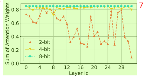
Figure 6: Sums of normalized attention weights for the selected tokens under different quantization precisions, with p = 0.85 .
