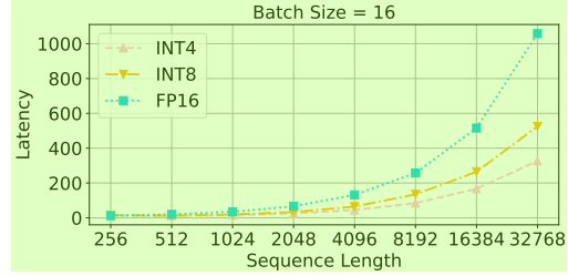
Figure 12: SpGEMV operator latency with different quantization bits. 5
