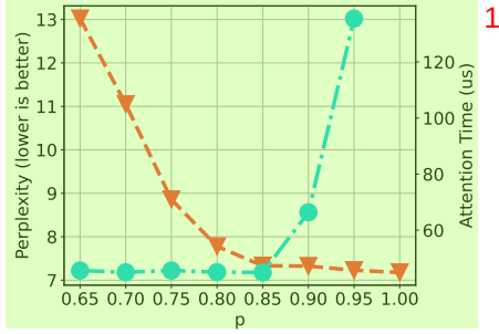
Figure 9: PG-19 perplexity (accuracy) and sparse attention latency (efficiency) under different threshold p values.
