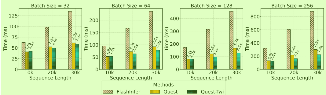
Figure 8: Time-Per-Output-Token (TPOT) improvements in end-to-end serving scenarios. 12
