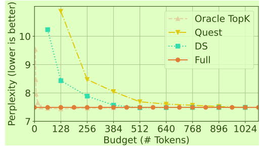
Figure 2: Relationship between the KV cache budget and the perplexity on the PG-19 dataset in different top- k sparse attention methods.
