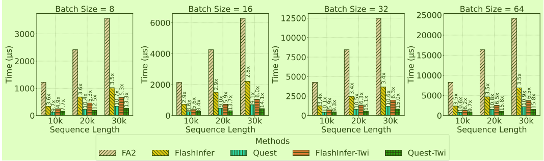
Figure 7: Latencies and speedups of self-attention at different sequence lengths and batch sizes. 6
