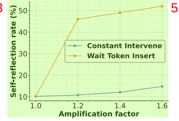
Figure 3: (c) Self-Reflection Ratio and Amplification Scale
