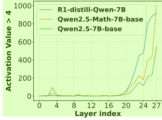
Figure 1: (a) Sparse Activations when processing Long CoT
