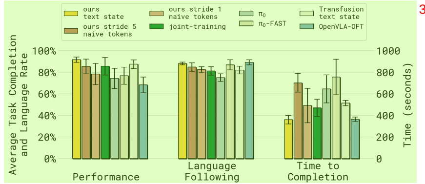
Figure 5: Comparison of multiple models/architectures on “table bussing” task with specialist models trained on a single robot embodiment. Our model has the highest performance, low inference time, and follows language instructions well. \pi_0 -FAST also follows language well and has good performance, but requires twice the amount of time (wall clock) to solve the task due to slow inference. \pi_0 struggles with following language instructions. OpenVLA-OFT follows language well and has low inference time, but has the lowest overall performance.
