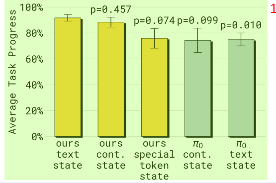
Figure 10: Comparison of different state representations on “table bussing” task. Our method works well with both text and continuous state, while \pi_0 works worse with both state representations. Therefore, the difference between \pi_0 and our method cannot be explained by the difference in their original state representations. Using special tokens as state performs worse.
