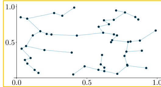
Figure 8: Example of the MST of a 2d uniformly sampled point cloud.
