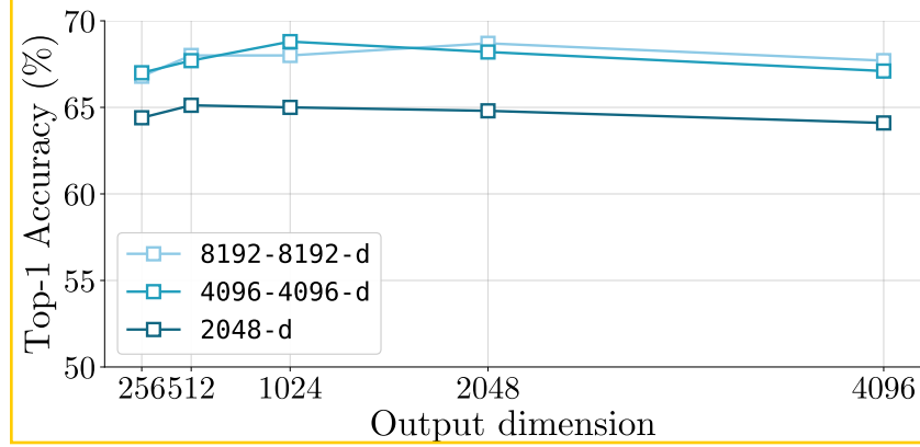
Figure 4: Impact of the projector architecture. \mathcal{L}_{\text{MSE}} + \mathcal{L}_{\text{TREGS}} top-1 accuracy (%) on the linear evaluation protocol with 100 pretraining epochs.
