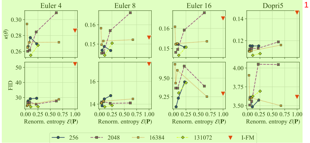
Figure 3: Experiment metrics for CIFAR-10 image generation. We evaluate the trained models using the Euler solver with three different number of steps, and with the Dopri5 solver and adaptive steps. The plots demonstrate the benefits of a larger OT batch size to achieve significantly smaller curvature, and moderately smaller FID at low number of integration steps. Our experiments also suggest that in this setting, lower renormalized entropy generally benefits the performance.
