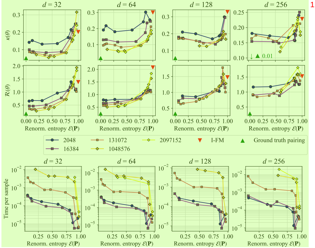
Figure 2: Results on the Korotin benchmark . As with Figure 1, we compute curvature and reconstruction metrics, and compute times below. Some of the runs for largest OT batch sizes n are provided in the supplementary. These runs suggest that to train OT models in these dimensions increasing n is overall beneficial across the board.
