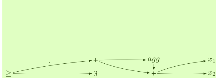
Figure 1: DAG data structure for the formula \text{agg}(x_1 + x_2) + (x_1 + x_2) \geq 3 .
