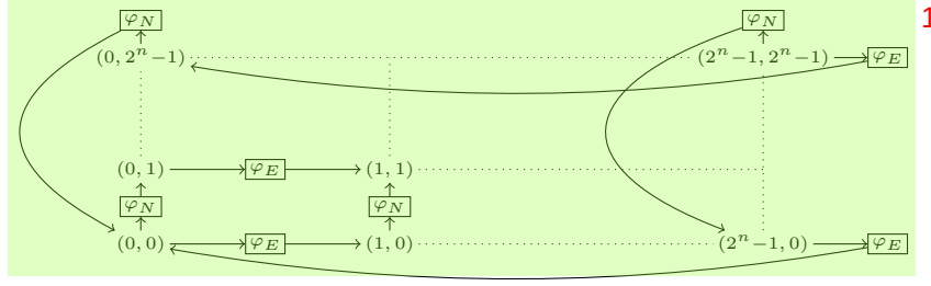
Figure 2: Encoding a torus of exponential size with (modal) q\mathcal{L} formulas. (x, y) are the vertices of the graph that correspond to locations in the torus while \varphi_N and \varphi_E denote intermediate vertices indicating the direction (resp., north and east).
