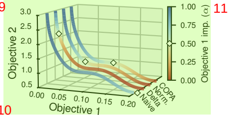
Figure 2: As we explore a synthetic Pareto front with different normalization functions to solve Eq. 3, only COPA meaningfully navigates it as we change \alpha , and its min-max solution agrees with our expectations of a robust solution.
