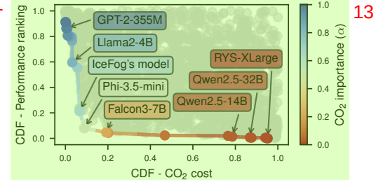
Figure 4: We can meaningfully explore the Pareto-optimal models of the Open LLM Leaderboard [12] with COPA. We use p = \infty on the 7 objectives and highlight some of the selected models as we change the value of \alpha .
