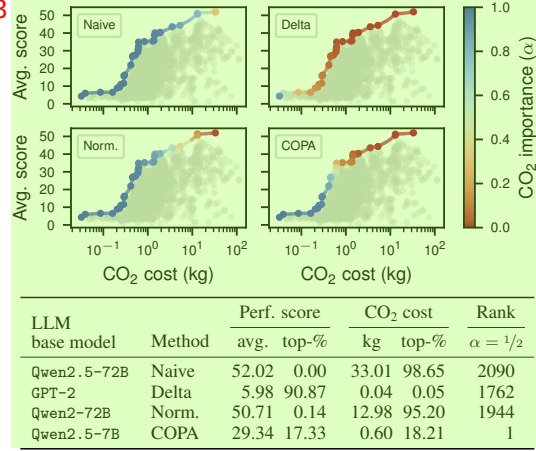
Figure 1: COPA meaningfully navigates the performance-emissions trade-off of the Open LLM Leaderboard [12], evenly mapping the importance of CO 2 cost to the Pareto front. In contrast, existing approaches are biased toward one of the objectives. This is reflected in the retrieved LLMs where, e.g., COPA maps \alpha = 1/2 to a top-18 % model for both objectives, and all other approaches select either a high-performing but CO 2 -demanding model, or vice versa.
