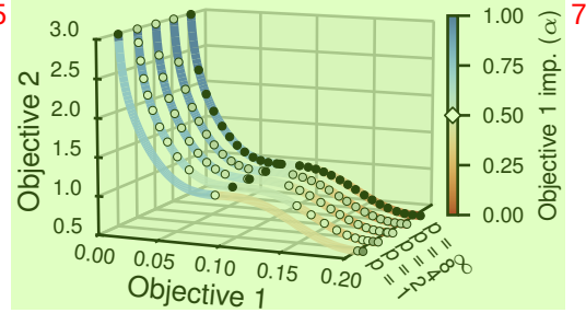
Figure 3: Distribution of solutions (circles) found for different values of p as we sweep over values of \alpha . The darkness of the circles represents the number of times they were selected.
