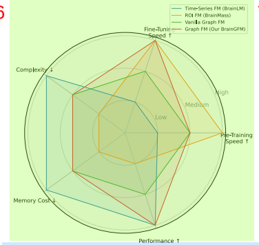
Figure 4: Comparison of performance and efficiency across different brain FMs.
